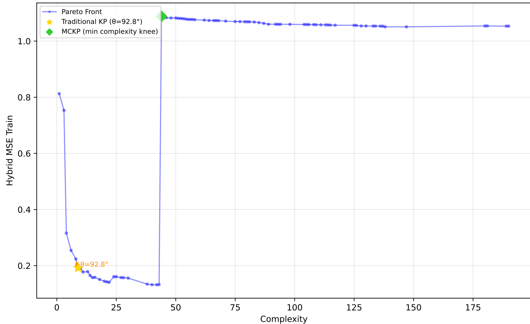
228_elusage - Run 10 - SVP - Hybrid MSE Train \lambda_1=0.00, \bar{\lambda}_2=1.00, \lambda_3=0.00 | Difficulty: 1.00 | Method: hmr
