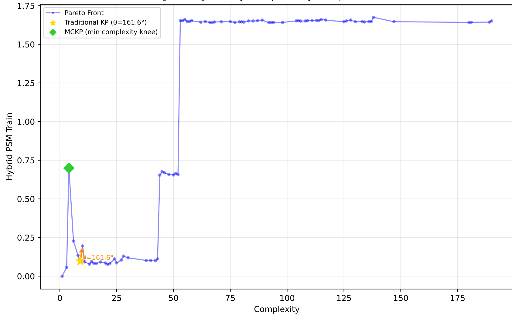
228_elusage - Run 10 - SVP - Hybrid PSM Train \lambda_1=0.60, \bar{\lambda}_2=0.60, \lambda_3=1.00 | Difficulty: 1.00 | Method: hmr
