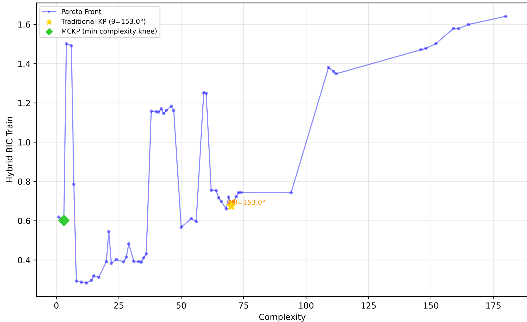
228_elusage - Run 11 - MVP - Hybrid BIC Train \lambda_1=0.00, \lambda_2=0.00, \lambda_3=1.00 | Difficulty: 1.00 | Method: hmr
