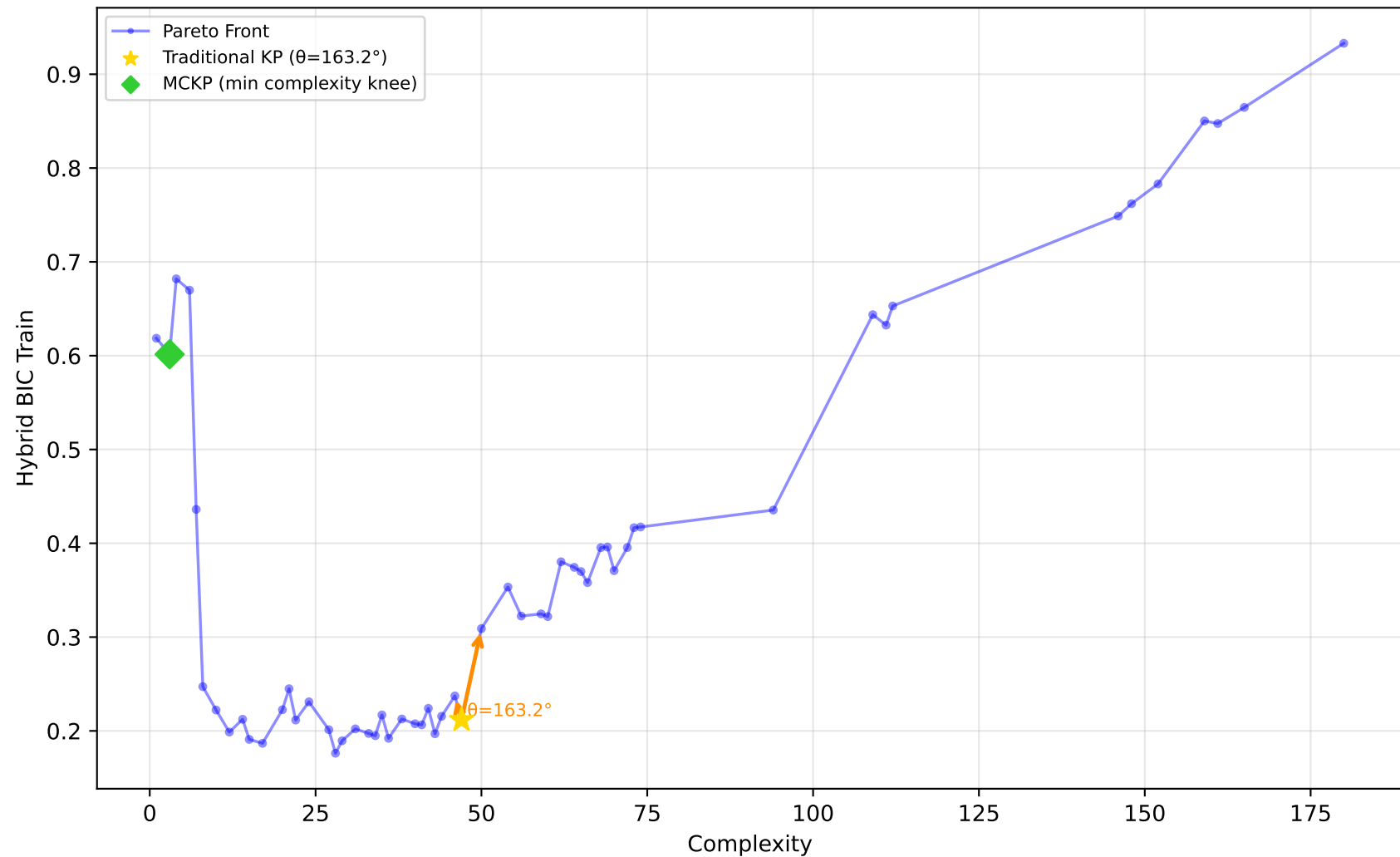
228_elusage - Run 11 - MVP - Hybrid BIC Train \lambda_1=0.00, \lambda_2=0.30, \lambda_3=0.00 | Difficulty: 1.00 | Method: hmr
