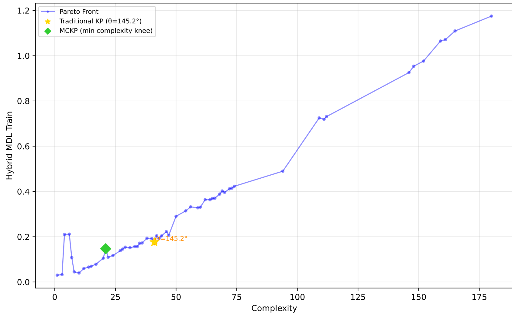
228_elusage - Run 11 - MVP - Hybrid MDL Train \lambda_1=0.00, \bar{\lambda}_2=0.30, \lambda_3=0.00 | Difficulty: 1.00 | Method: hmr
