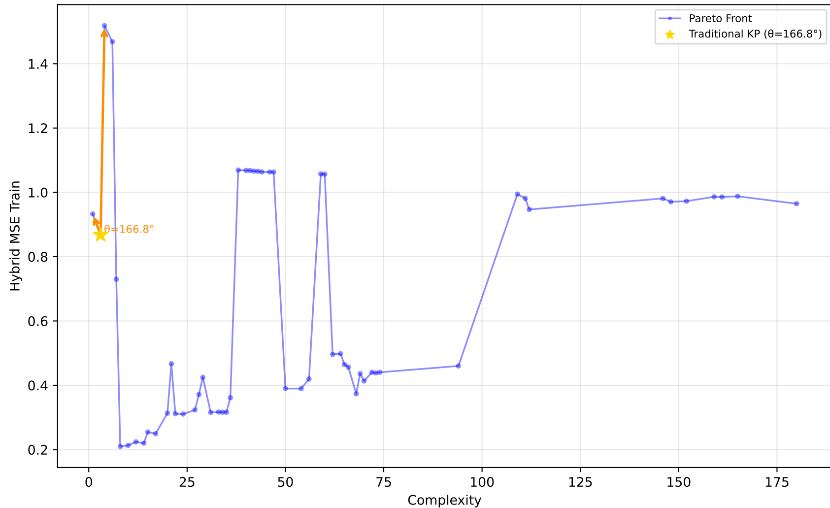
228_elusage - Run 11 - MVP - Hybrid MSE Train \lambda_1=0.00, \bar{\lambda}_2=0.00, \lambda_3=1.00 | Difficulty: 1.00 | Method: hmr
