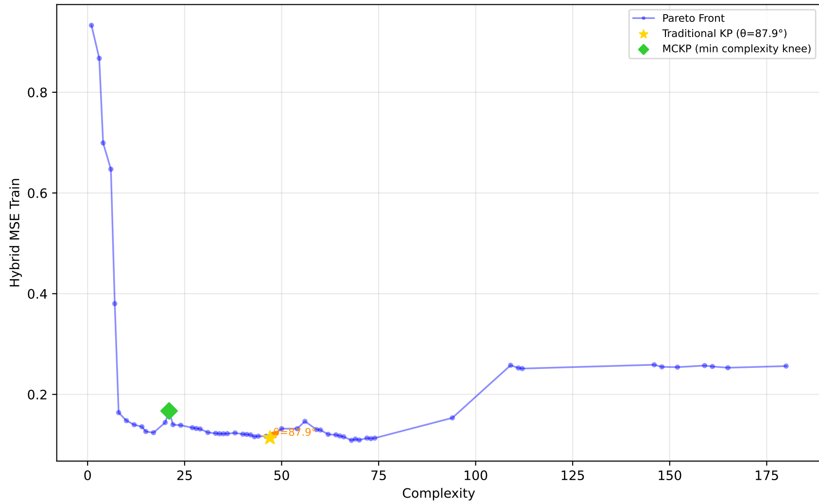
228_elusage - Run 11 - MVP - Hybrid MSE Train \lambda_1=0.00, \bar{\lambda}_2=0.30, \lambda_3=0.00 | Difficulty: 1.00 | Method: hmr
