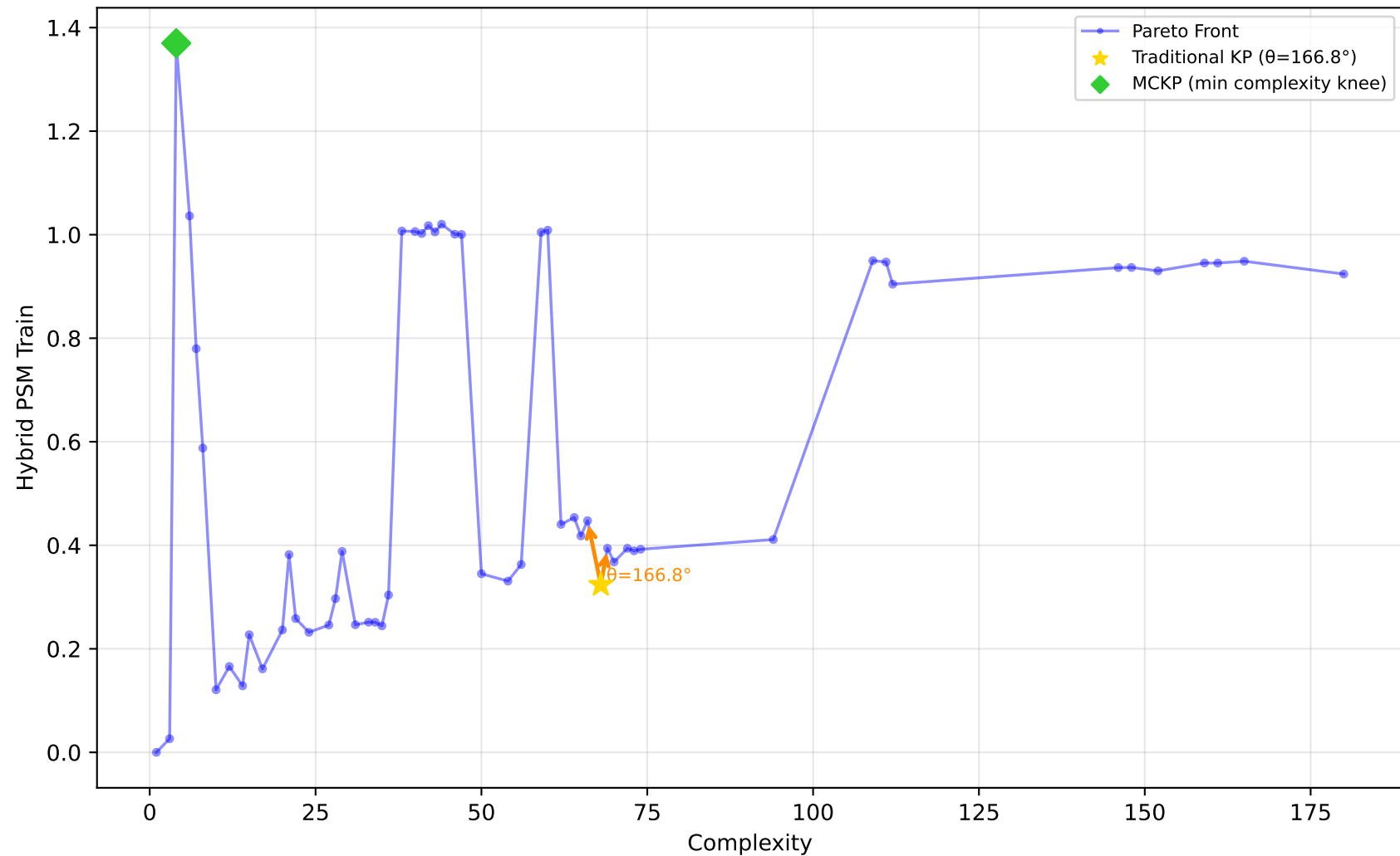
228_elusage - Run 11 - MVP - Hybrid PSM Train \lambda_1=0.00, \bar{\lambda}_2=0.00, \lambda_3=1.00 | Difficulty: 1.00 | Method: hmr
