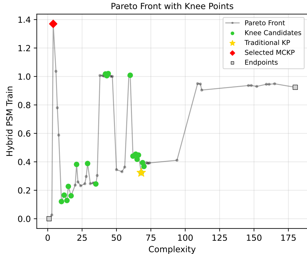
228_elusage - Run 11 - MVP - Hybrid PSM Train - Clustering Threshold \lambda_1=0.00, \lambda_2=0.00, \lambda_3=1.00 | Difficulty: 1.00
