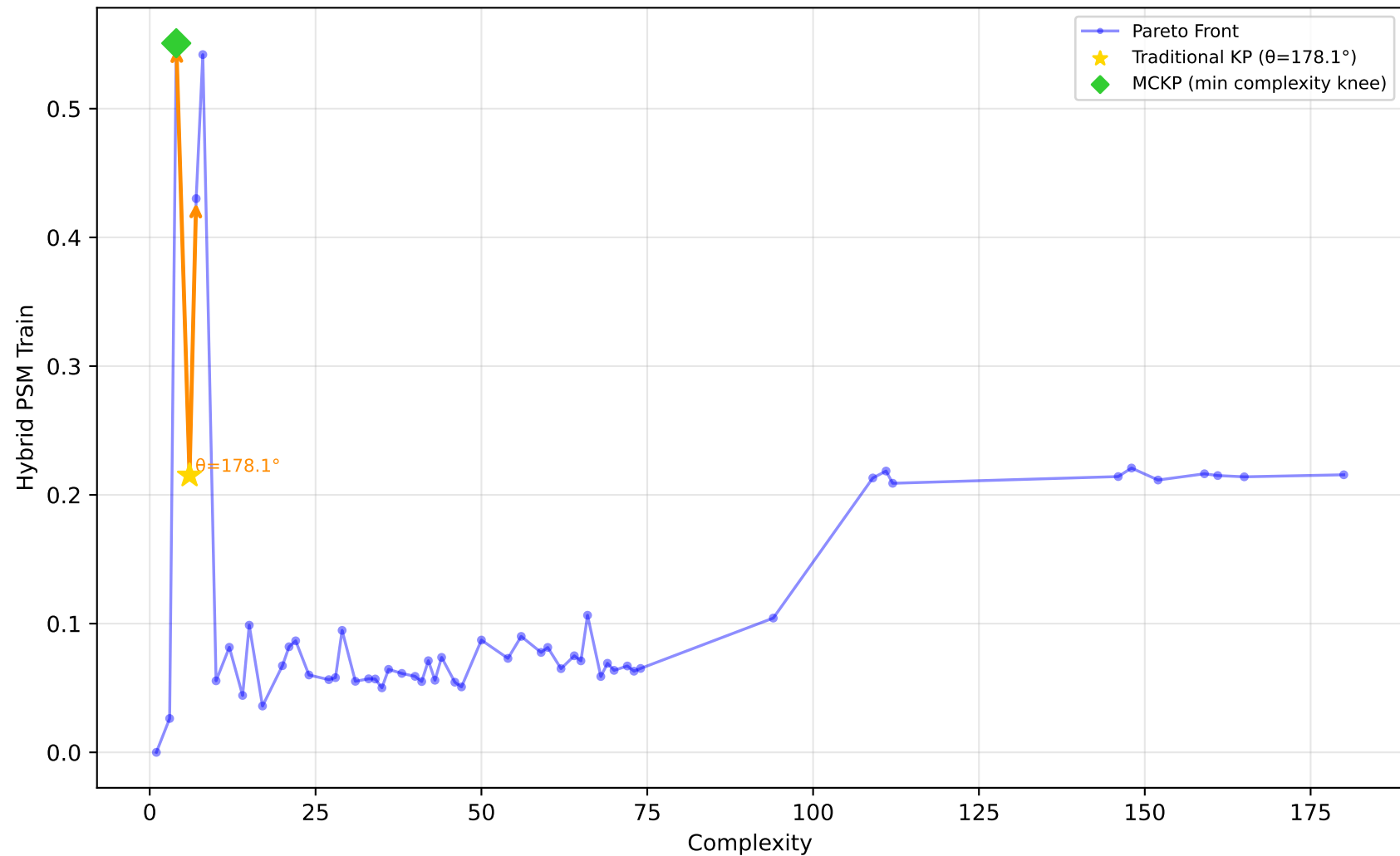
228_elusage - Run 11 - MVP - Hybrid PSM Train \lambda_1=0.00, \bar{\lambda}_2=0.30, \lambda_3=0.00 | Difficulty: 1.00 | Method: hmr
