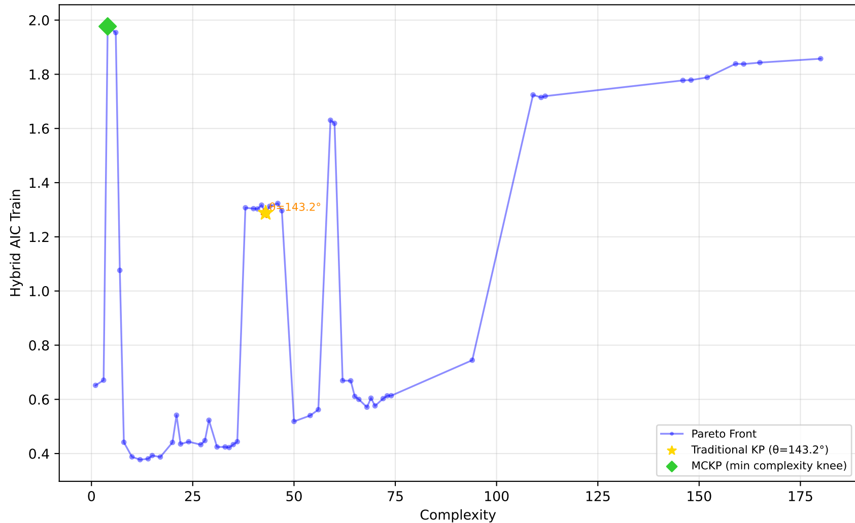
228_elusage - Run 11 - SVP - Hybrid AIC Train \lambda_1=0.60, \lambda_2=0.60, \lambda_3=1.00 | Difficulty: 1.00 | Method: hmr
