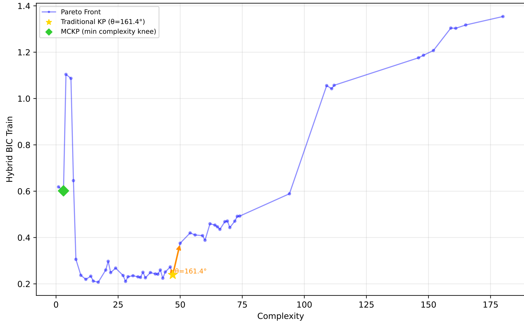
228_elusage - Run 11 - SVP - Hybrid BIC Train \lambda_1=0.00, \lambda_2=1.00, \lambda_3=0.00 | Difficulty: 1.00 | Method: hmr
