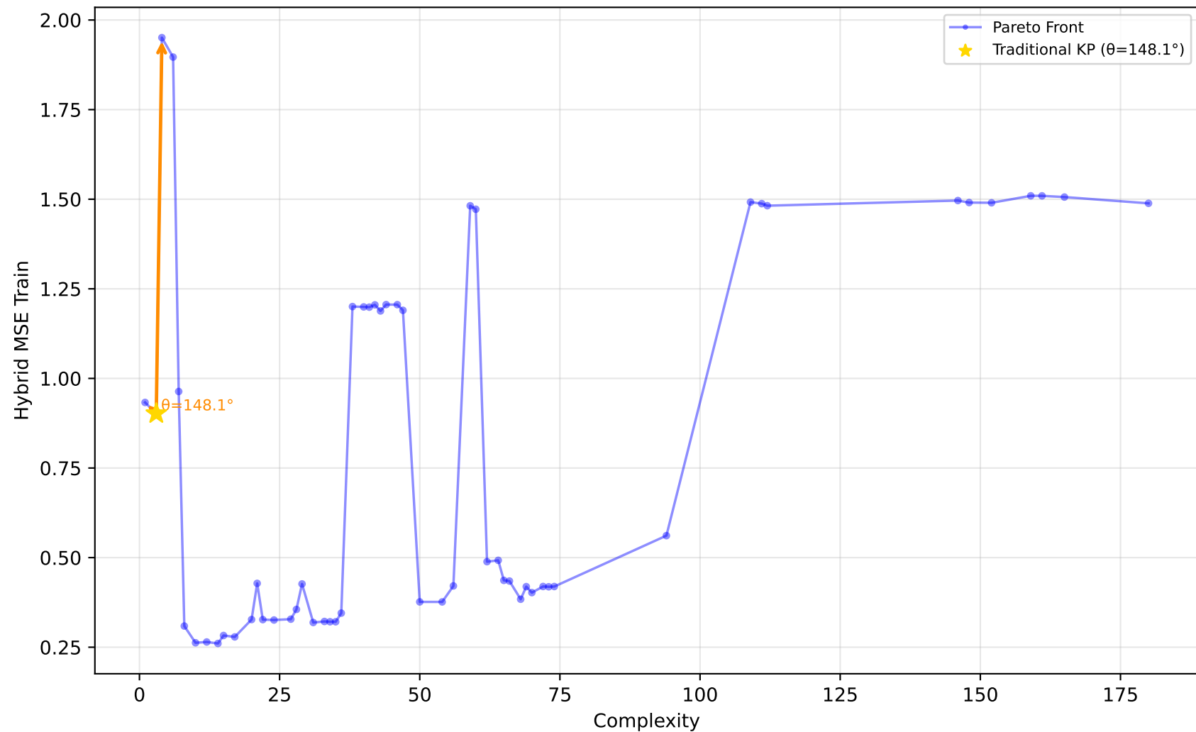
228_elusage - Run 11 - SVP - Hybrid MSE Train \lambda_1=0.60, \bar{\lambda}_2=0.60, \lambda_3=1.00 | Difficulty: 1.00 | Method: hmr
