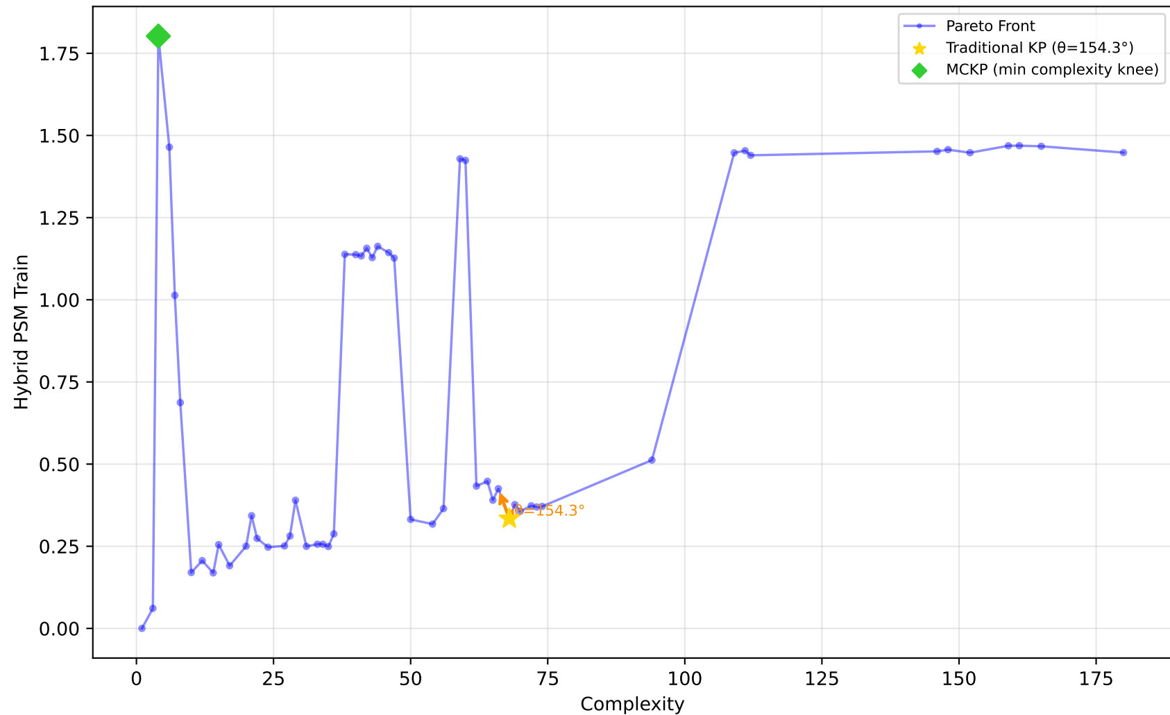
228_elusage - Run 11 - SVP - Hybrid PSM Train \lambda_1=0.60, \bar{\lambda}_2=0.60, \lambda_3=1.00 | Difficulty: 1.00 | Method: hmr
