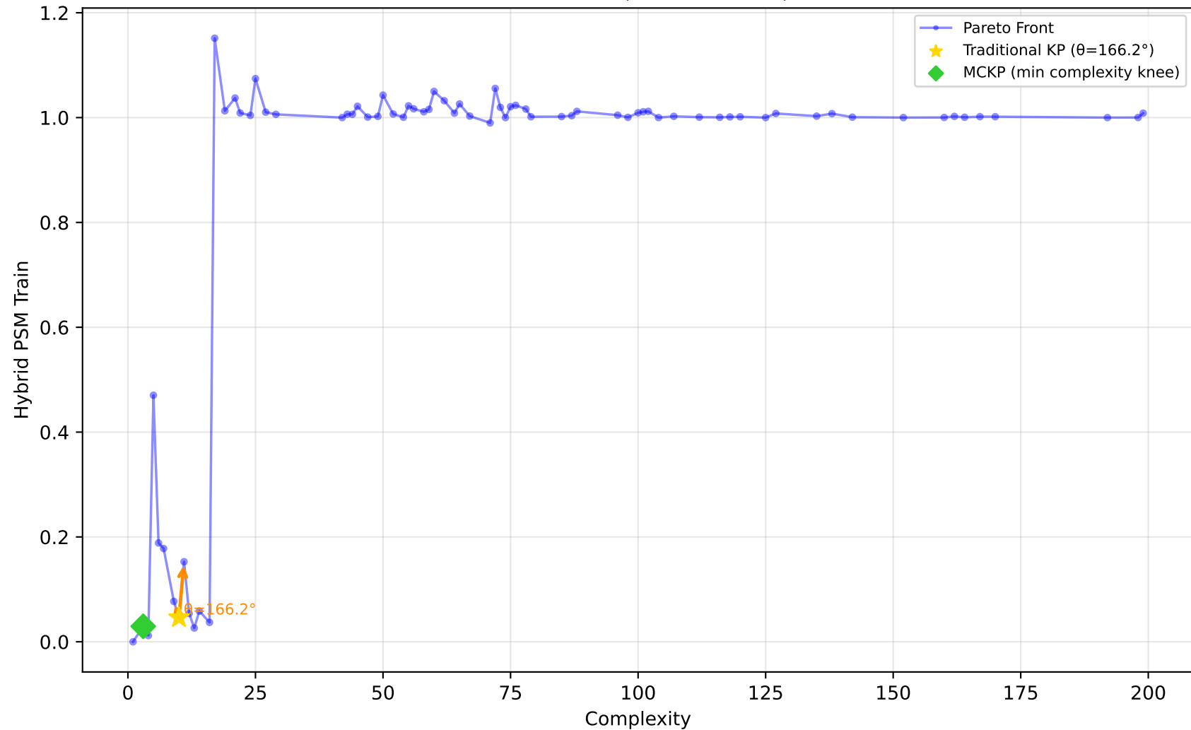
228_elusage - Run 12 - MVP - Hybrid PSM Train \lambda_1=0.00, \bar{\lambda}_2=0.00, \lambda_3=1.00 | Difficulty: 1.00 | Method: hmr
