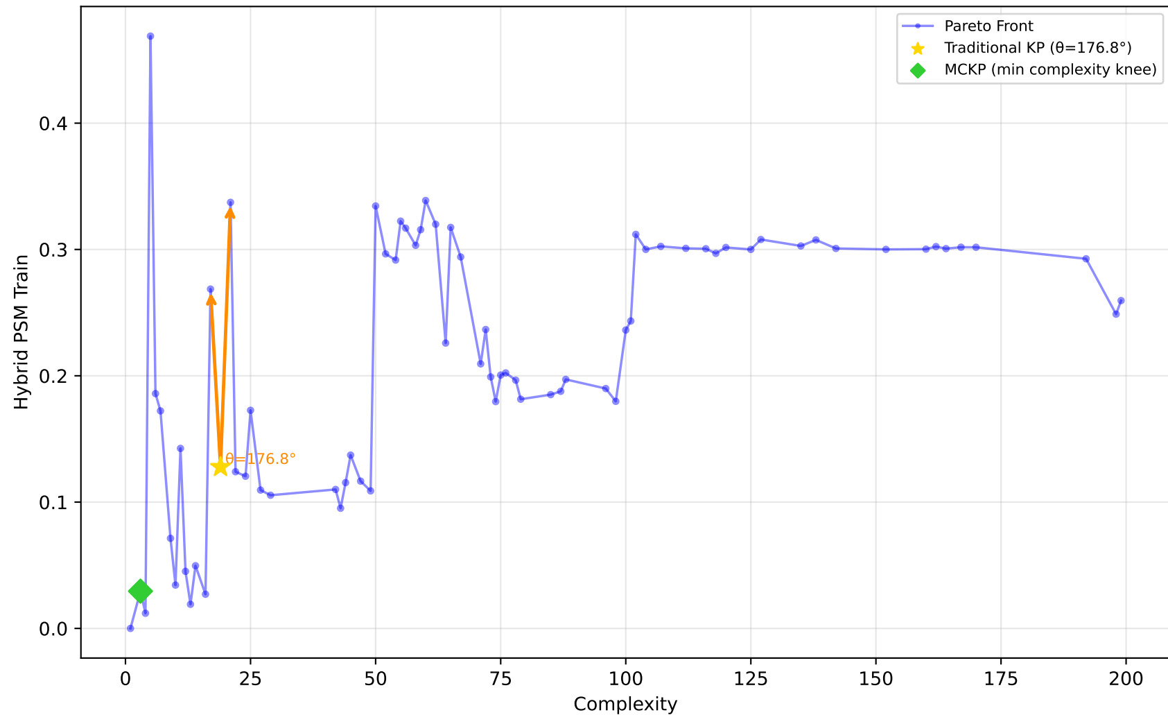
228_elusage - Run 12 - MVP - Hybrid PSM Train \lambda_1=0.00, \bar{\lambda}_2=0.30, \lambda_3=0.00 | Difficulty: 1.00 | Method: hmr
