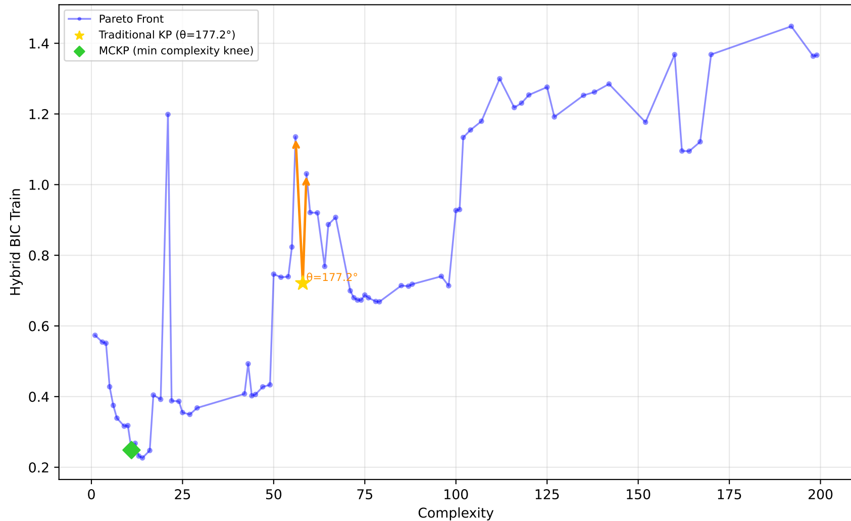
228_elusage - Run 12 - SVP - Hybrid BIC Train \lambda_1=0.00, \lambda_2=1.00, \lambda_3=0.00 | Difficulty: 1.00 | Method: hmr
