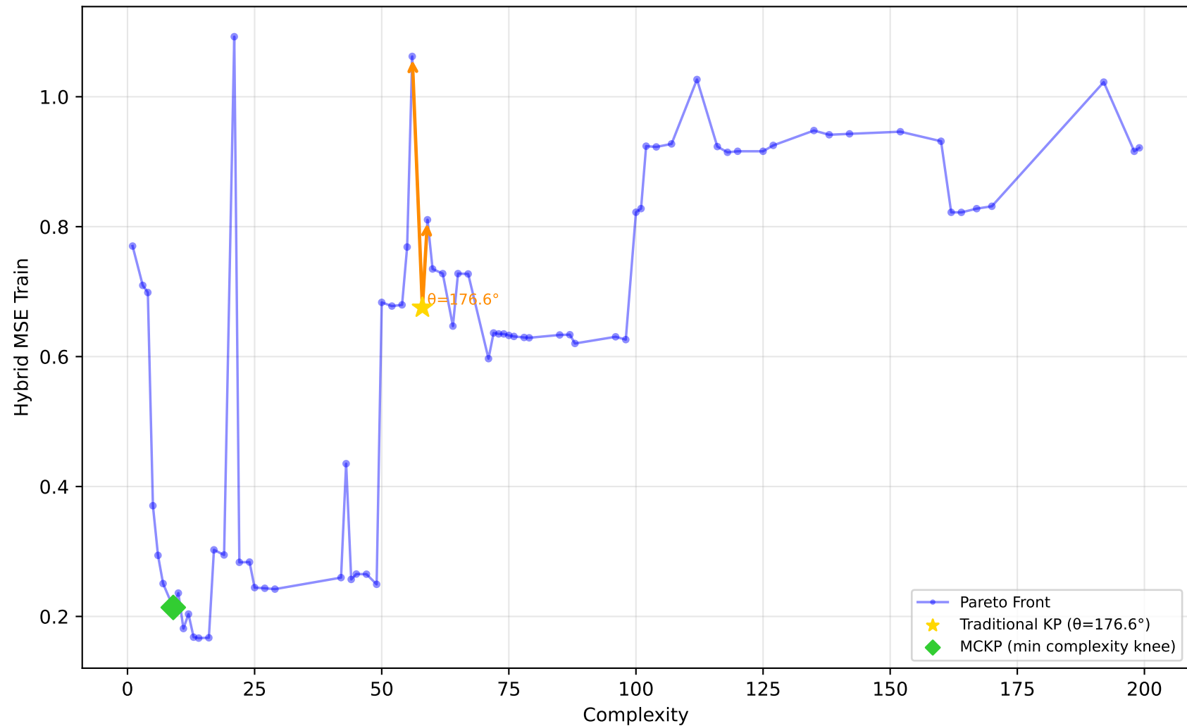
228_elusage - Run 12 - SVP - Hybrid MSE Train \lambda_1=0.00, \bar{\lambda}_2=1.00, \lambda_3=0.00 | Difficulty: 1.00 | Method: hmr
