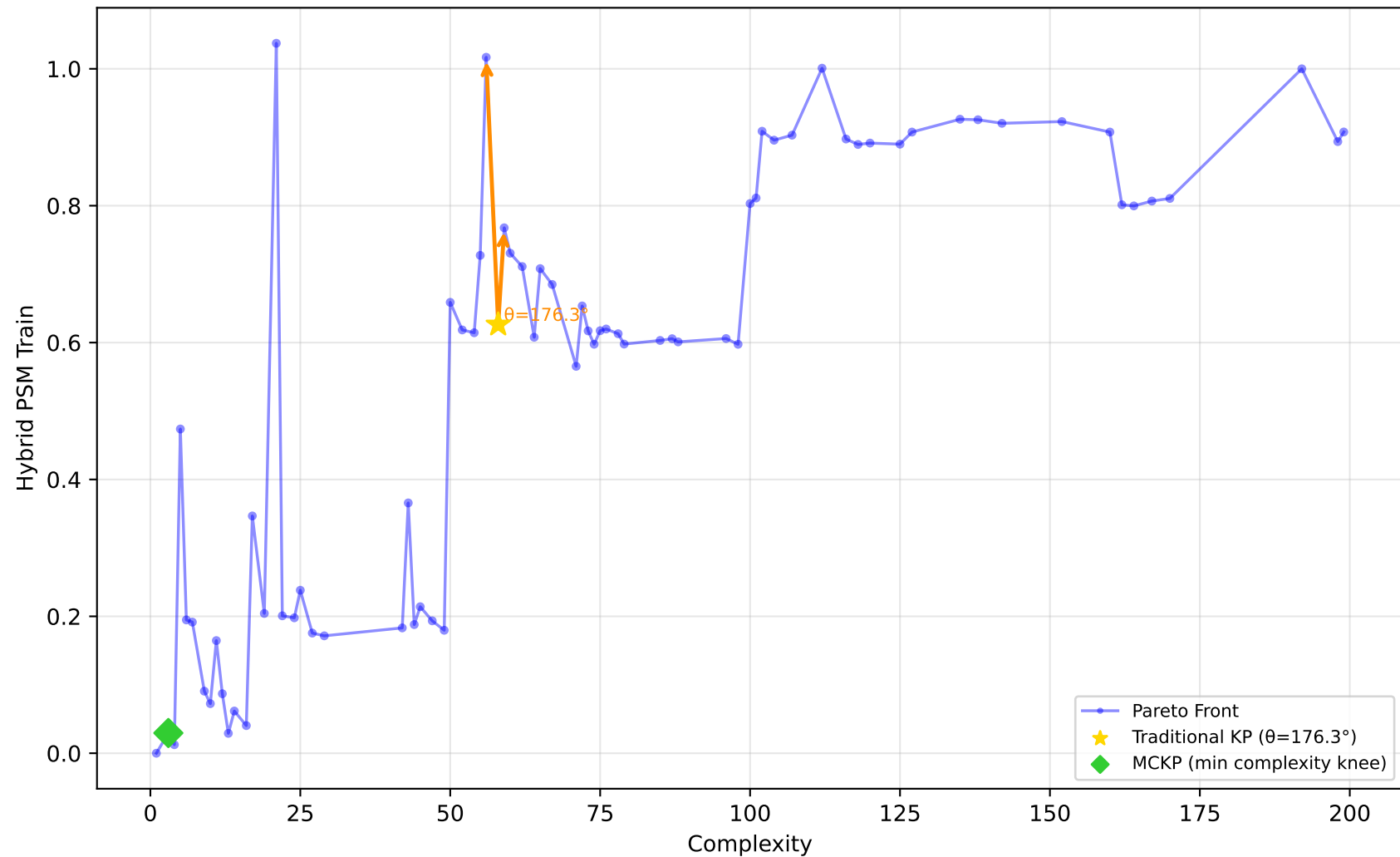
228_elusage - Run 12 - SVP - Hybrid PSM Train \lambda_1=0.00, \bar{\lambda}_2=1.00, \lambda_3=0.00 | Difficulty: 1.00 | Method: hmr
