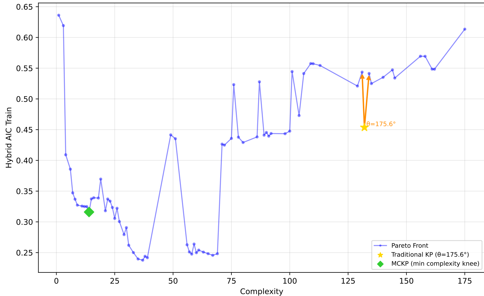
228_elusage - Run 13 - MVP - Hybrid AIC Train \lambda_1=0.00, \lambda_2=0.30, \lambda_3=0.00 | Difficulty: 1.00 | Method: hmr
