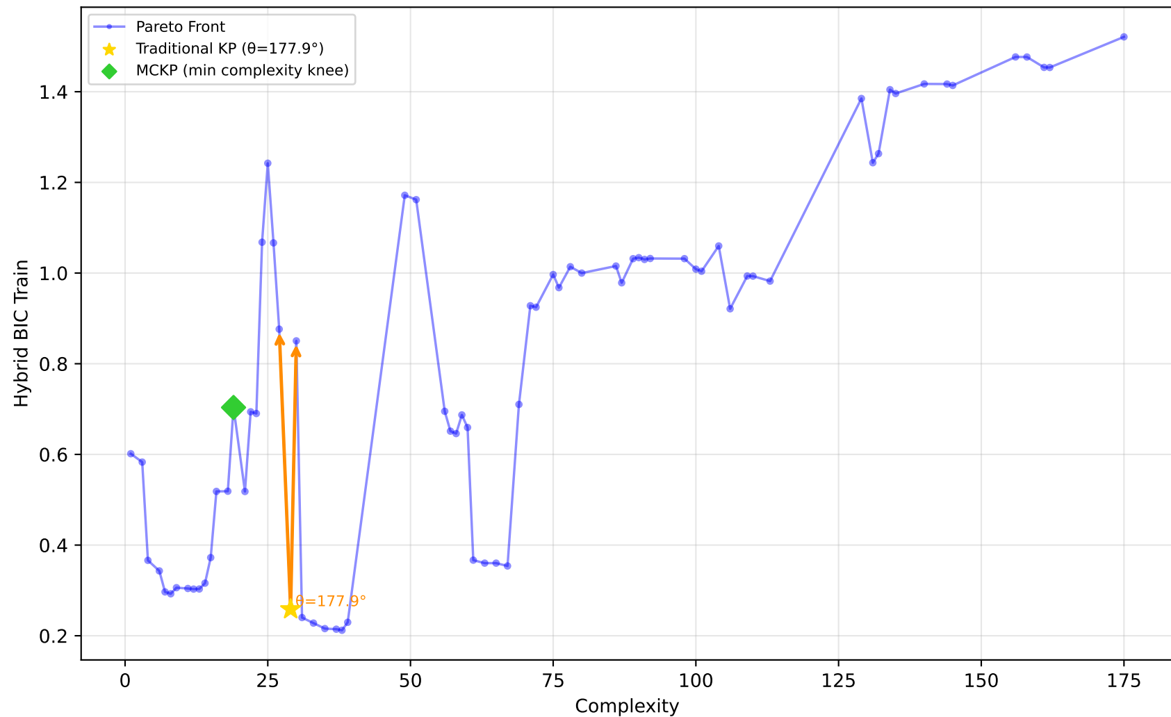
228_elusage - Run 13 - MVP - Hybrid BIC Train \lambda_1=0.00, \lambda_2=0.00, \lambda_3=1.00 | Difficulty: 1.00 | Method: hmr
