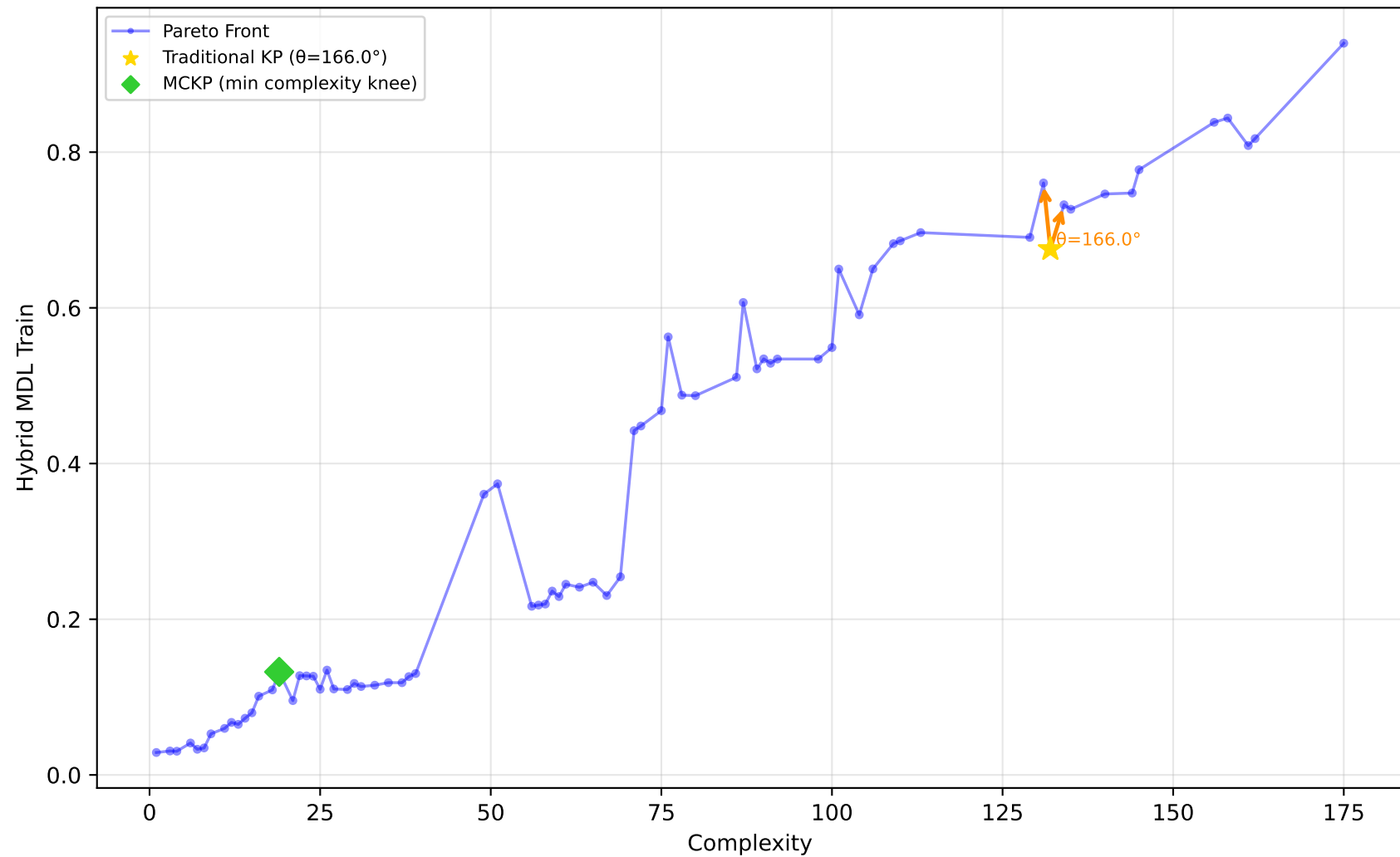
228_elusage - Run 13 - MVP - Hybrid MDL Train \lambda_1=0.00, \bar{\lambda}_2=0.30, \lambda_3=0.00 | Difficulty: 1.00 | Method: hmr
