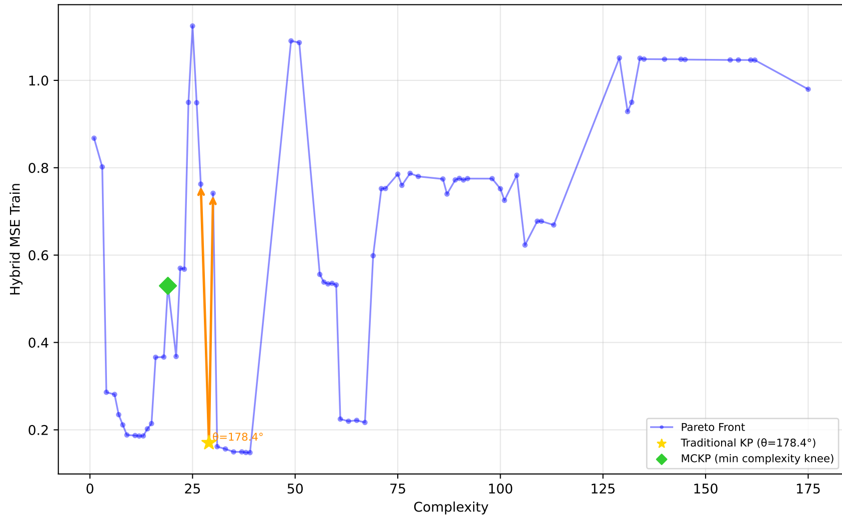
228_elusage - Run 13 - MVP - Hybrid MSE Train \lambda_1=0.00, \bar{\lambda}_2=0.00, \lambda_3=1.00 | Difficulty: 1.00 | Method: hmr
