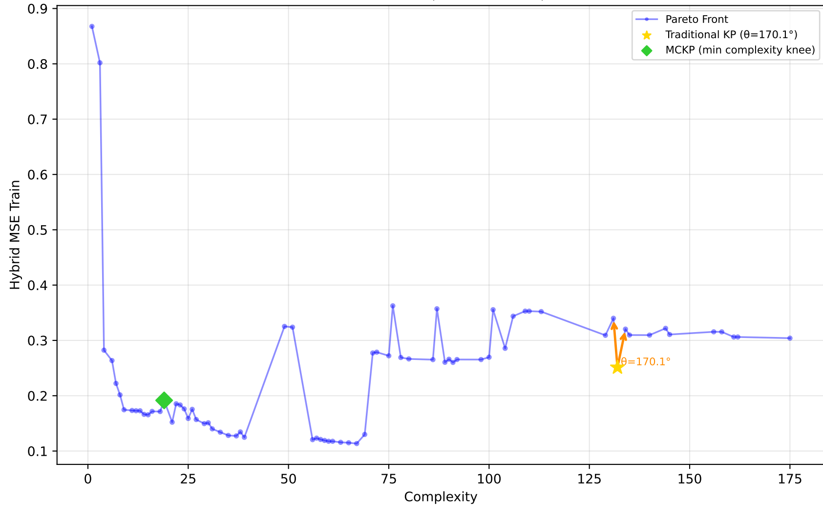
228_elusage - Run 13 - MVP - Hybrid MSE Train \lambda_1=0.00, \bar{\lambda}_2=0.30, \lambda_3=0.00 | Difficulty: 1.00 | Method: hmr
