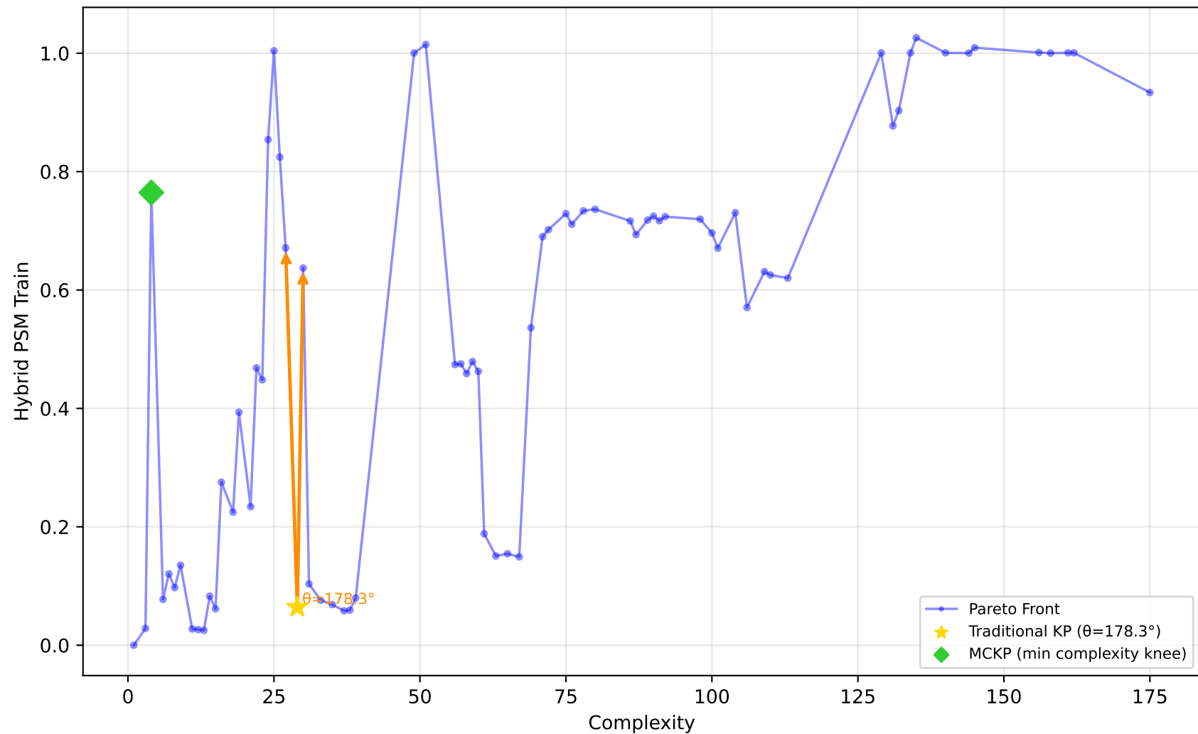
228_elusage - Run 13 - MVP - Hybrid PSM Train \lambda_1=0.00, \bar{\lambda}_2=0.00, \lambda_3=1.00 | Difficulty: 1.00 | Method: hmr
