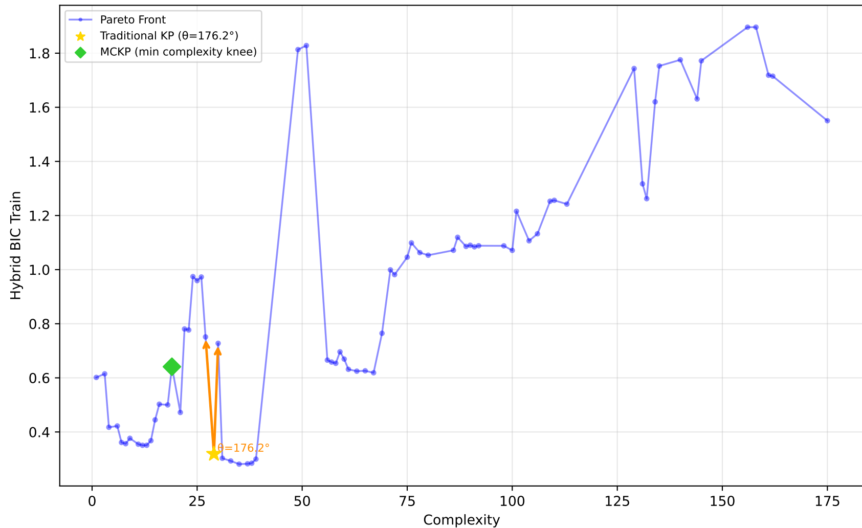
228_elusage - Run 13 - SVP - Hybrid BIC Train \lambda_1=0.60, \lambda_2=0.60, \lambda_3=1.00 | Difficulty: 1.00 | Method: hmr
