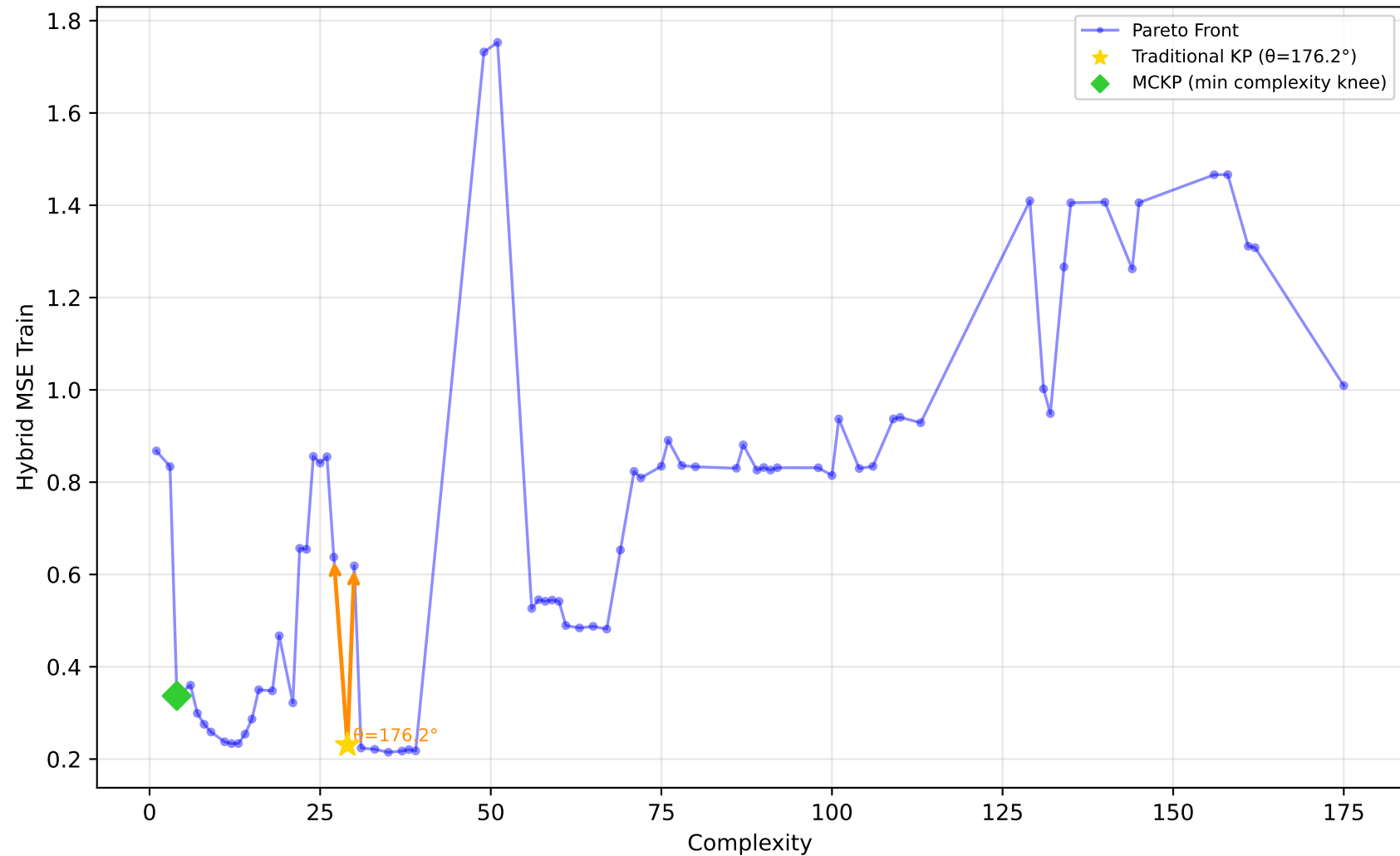
228_elusage - Run 13 - SVP - Hybrid MSE Train \lambda_1=0.60, \bar{\lambda}_2=0.60, \lambda_3=1.00 | Difficulty: 1.00 | Method: hmr
