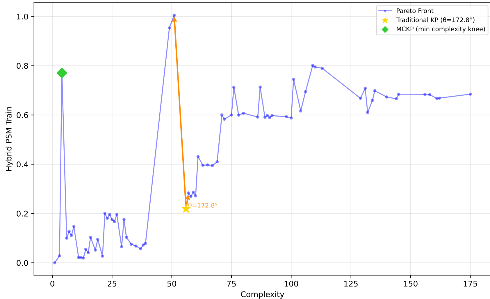
228_elusage - Run 13 - SVP - Hybrid PSM Train \lambda_1=0.00, \bar{\lambda}_2=1.00, \lambda_3=0.00 | Difficulty: 1.00 | Method: hmr
