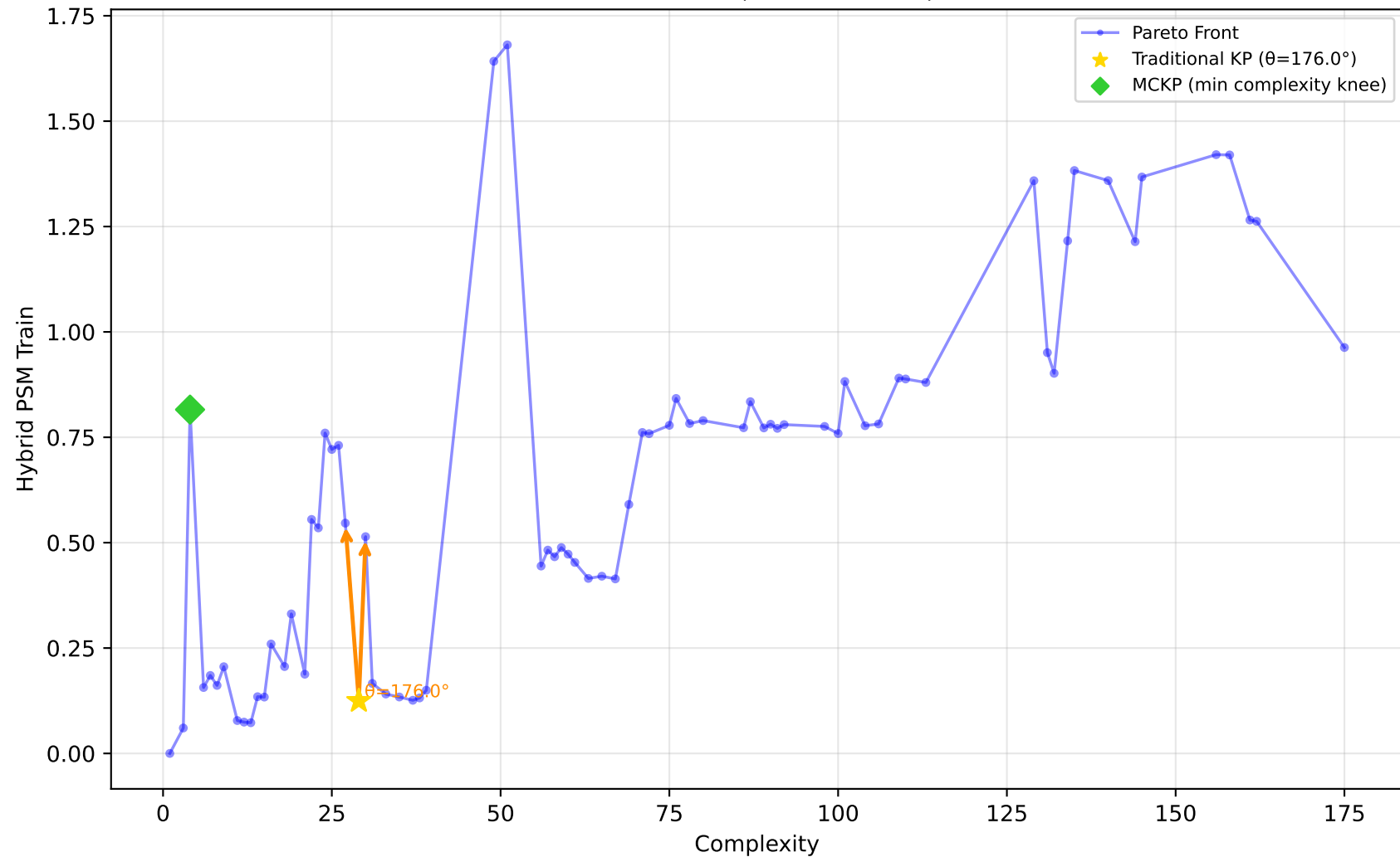
228_elusage - Run 13 - SVP - Hybrid PSM Train \lambda_1=0.60, \bar{\lambda}_2=0.60, \lambda_3=1.00 | Difficulty: 1.00 | Method: hmr
