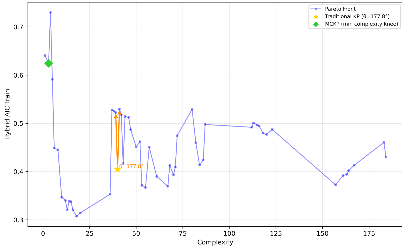
228_elusage - Run 14 - MVP - Hybrid AIC Train \lambda_1=0.00, \lambda_2=0.30, \lambda_3=0.00 | Difficulty: 1.00 | Method: hmr
