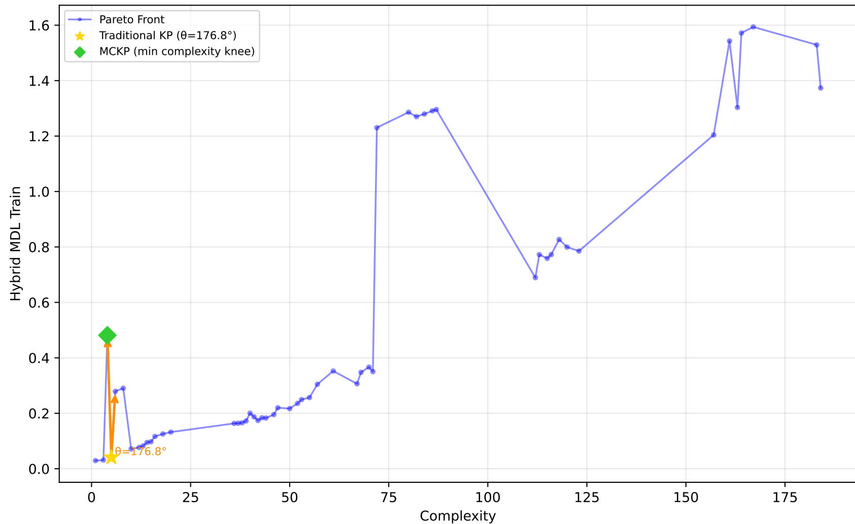
228_elusage - Run 14 - MVP - Hybrid MDL Train \lambda_1=0.00, \bar{\lambda}_2=0.00, \lambda_3=1.00 | Difficulty: 1.00 | Method: hmr
