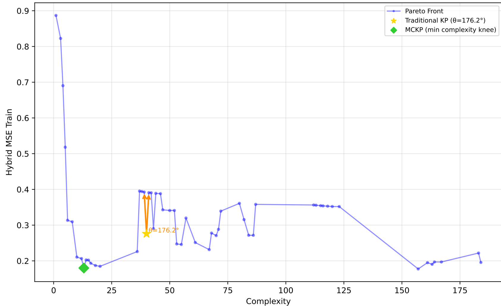
228_elusage - Run 14 - MVP - Hybrid MSE Train \lambda_1=0.00, \bar{\lambda}_2=0.30, \lambda_3=0.00 | Difficulty: 1.00 | Method: hmr
