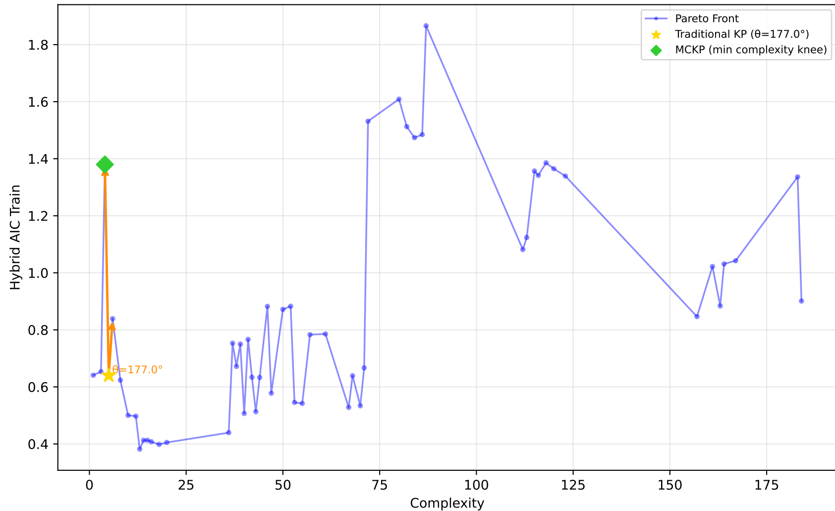
228_elusage - Run 14 - SVP - Hybrid AIC Train \lambda_1=0.60, \lambda_2=0.60, \lambda_3=1.00 | Difficulty: 1.00 | Method: hmr
