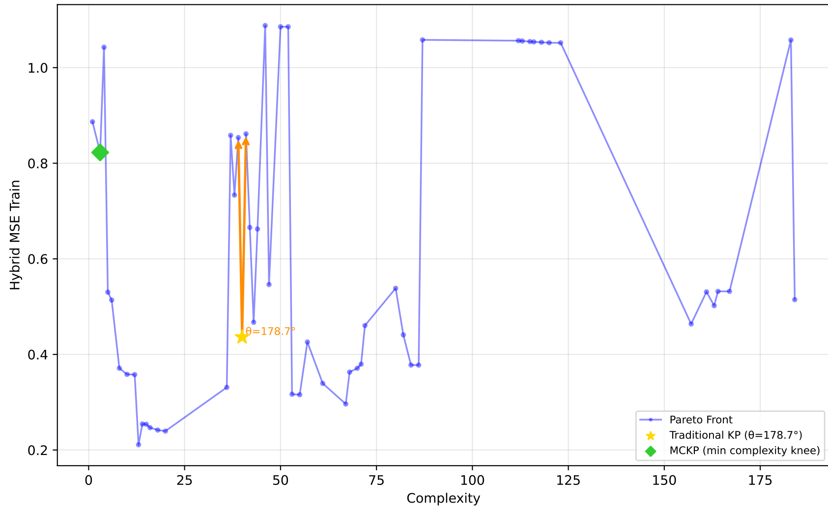
228_elusage - Run 14 - SVP - Hybrid MSE Train \lambda_1=0.00, \bar{\lambda}_2=1.00, \lambda_3=0.00 | Difficulty: 1.00 | Method: hmr
