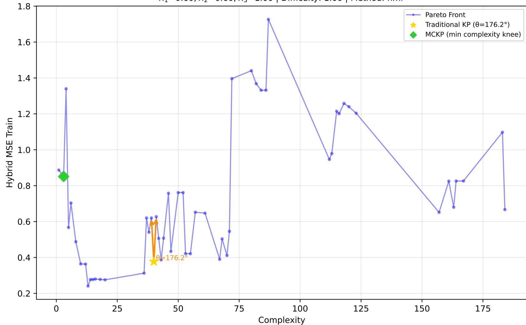
228_elusage - Run 14 - SVP - Hybrid MSE Train \lambda_1=0.60, \bar{\lambda}_2=0.60, \lambda_3=1.00 | Difficulty: 1.00 | Method: hmr
