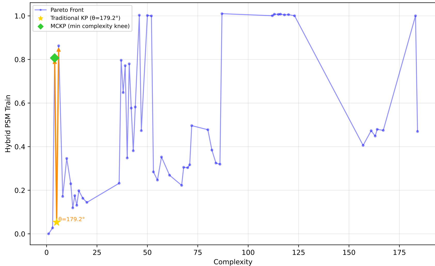
228_elusage - Run 14 - SVP - Hybrid PSM Train \lambda_1=0.00, \bar{\lambda}_2=1.00, \lambda_3=0.00 | Difficulty: 1.00 | Method: hmr
