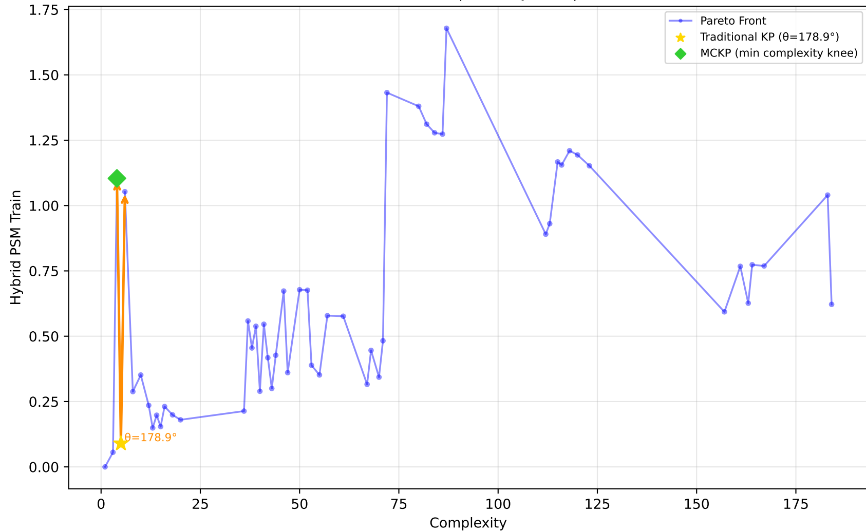
228_elusage - Run 14 - SVP - Hybrid PSM Train \lambda_1=0.60, \bar{\lambda}_2=0.60, \lambda_3=1.00 | Difficulty: 1.00 | Method: hmr
