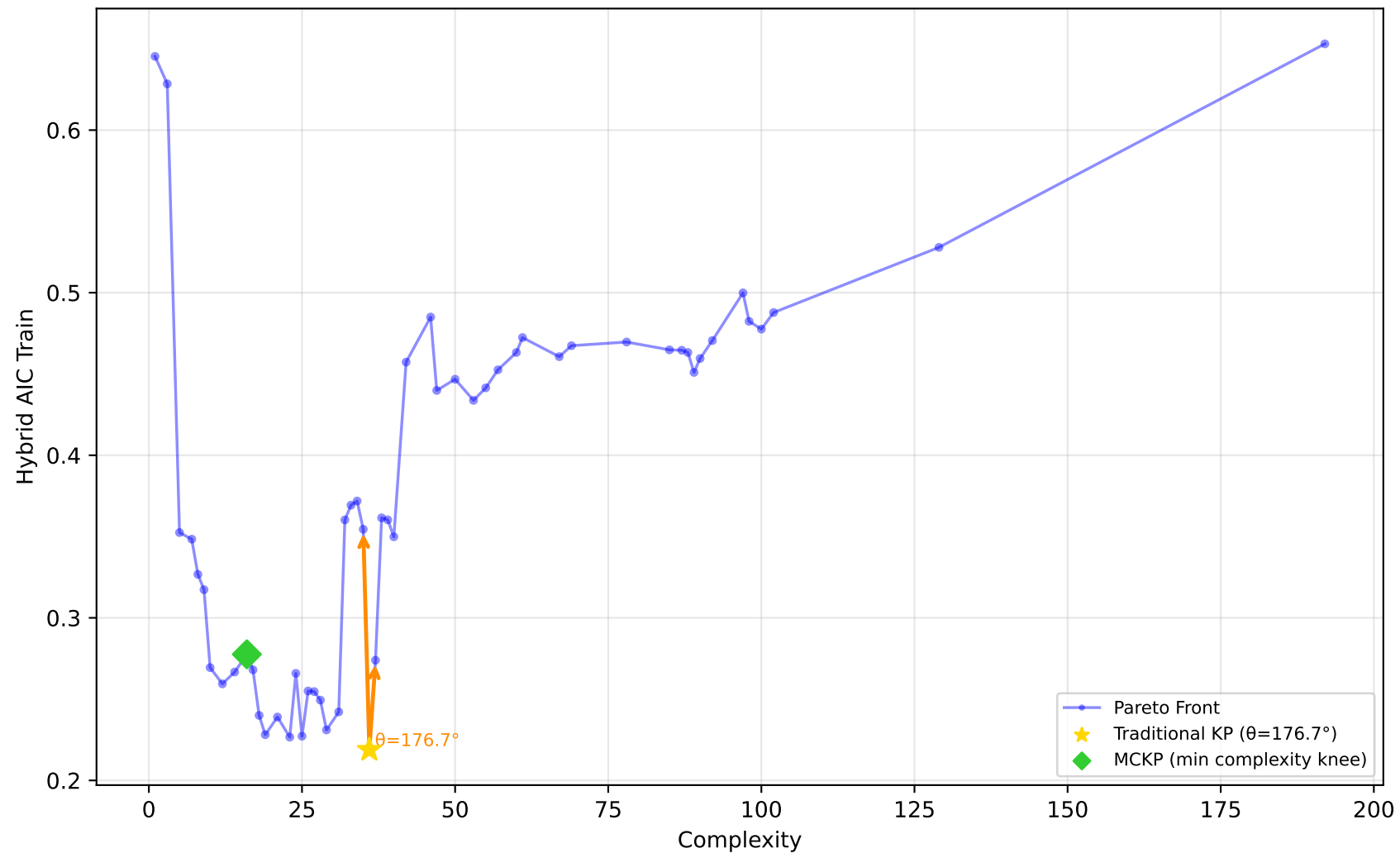
228_elusage - Run 15 - MVP - Hybrid AIC Train \lambda_1=0.00, \bar{\lambda}_2=0.30, \lambda_3=0.00 | Difficulty: 0.66 | Method: hmr
