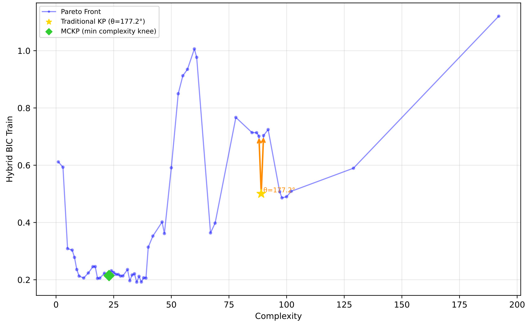
228_elusage - Run 15 - MVP - Hybrid BIC Train \lambda_1=0.00, \bar{\lambda}_2=0.00, \lambda_3=1.00 | Difficulty: 0.66 | Method: hmr
