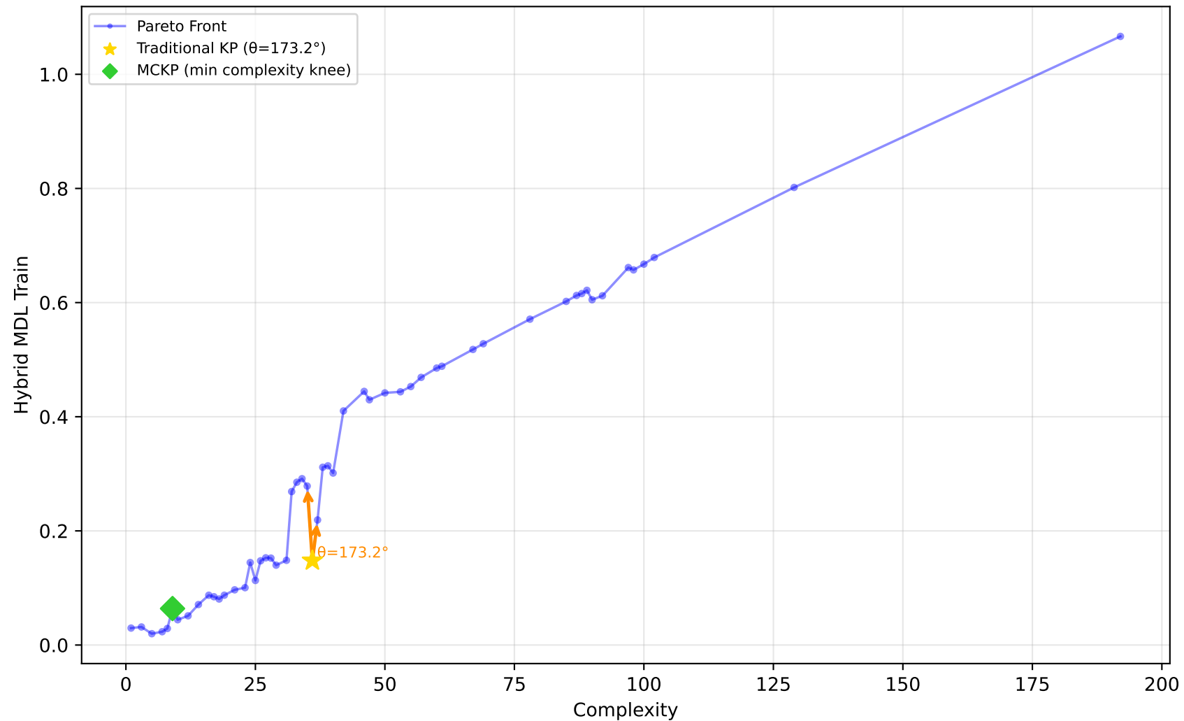
228_elusage - Run 15 - MVP - Hybrid MDL Train \lambda_1=0.00, \bar{\lambda}_2=0.30, \lambda_3=0.00 | Difficulty: 0.66 | Method: hmr
