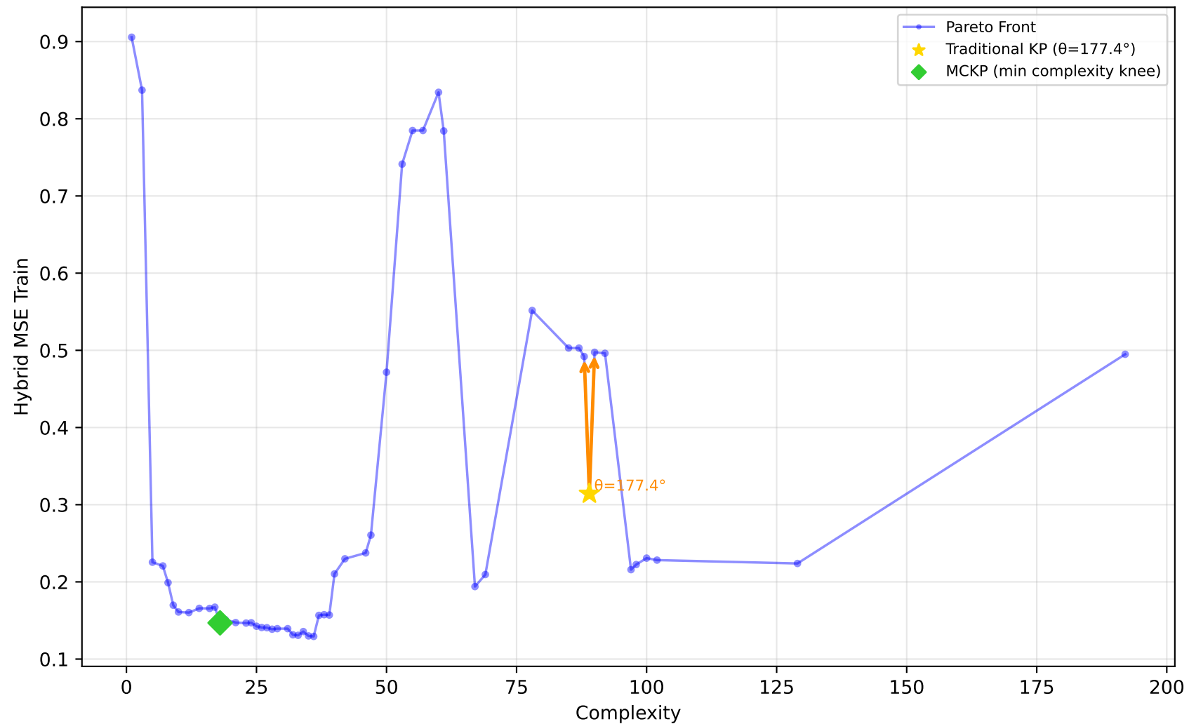
228 elusage - Run 15 - MVP - Hybrid MSE Train \lambda_1=0.00, \bar{\lambda}_2=0.00, \lambda_3=1.00 | Difficulty: 0.66 | Method: hmr
