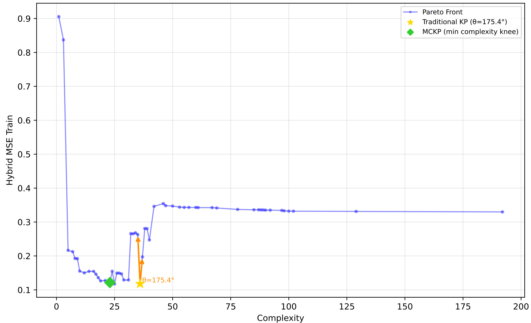
228_elusage - Run 15 - MVP - Hybrid MSE Train \lambda_1=0.00, \bar{\lambda}_2=0.30, \lambda_3=0.00 | Difficulty: 0.66 | Method: hmr
