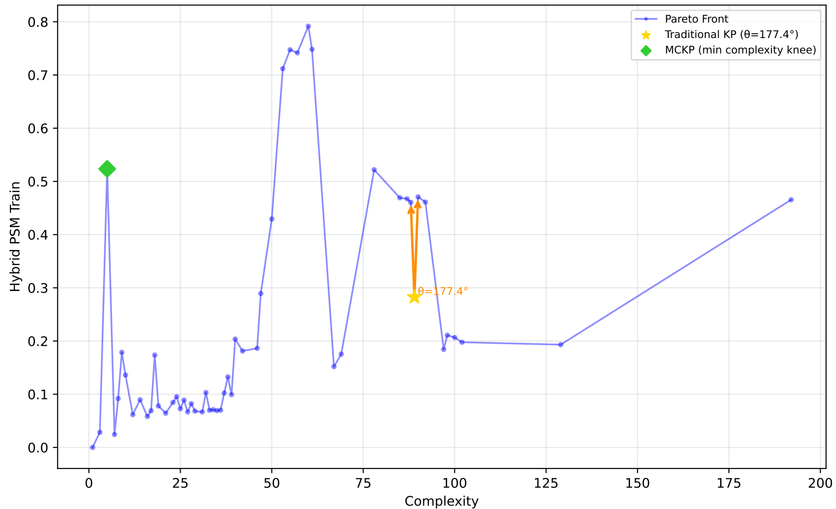
228_elusage - Run 15 - MVP - Hybrid PSM Train \lambda_1=0.00, \bar{\lambda}_2=0.00, \lambda_3=1.00 | Difficulty: 0.66 | Method: hmr
