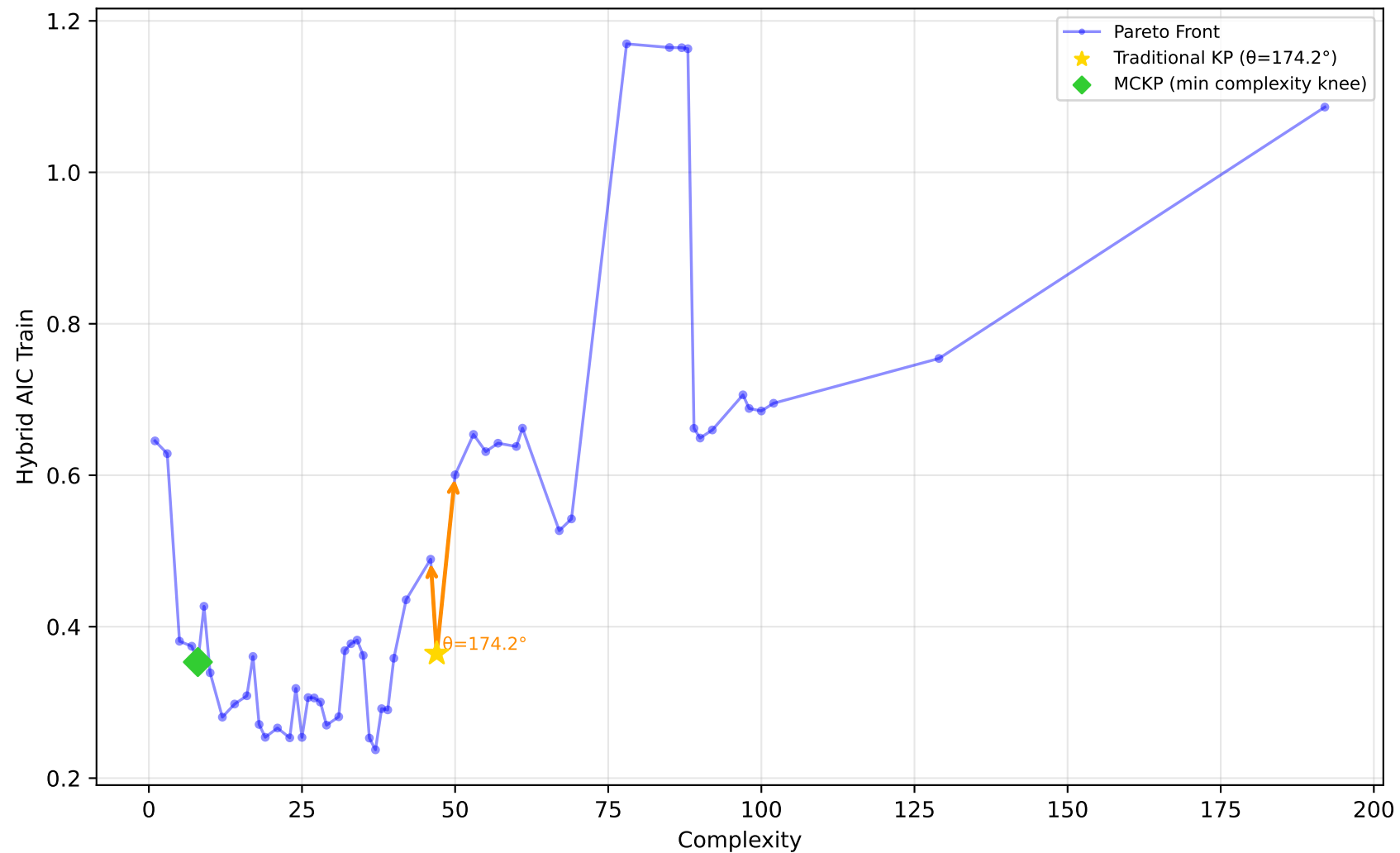
228_elusage - Run 15 - SVP - Hybrid AIC Train \lambda_1=0.00, \lambda_2=1.00, \lambda_3=0.00 | Difficulty: 0.66 | Method: hmr
