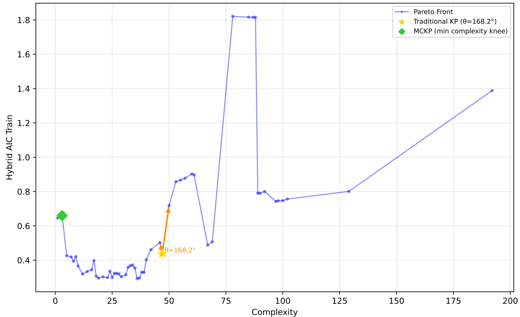
228_elusage - Run 15 - SVP - Hybrid AIC Train \lambda_1=0.60, \lambda_2=0.60, \lambda_3=1.00 | Difficulty: 0.66 | Method: hmr
