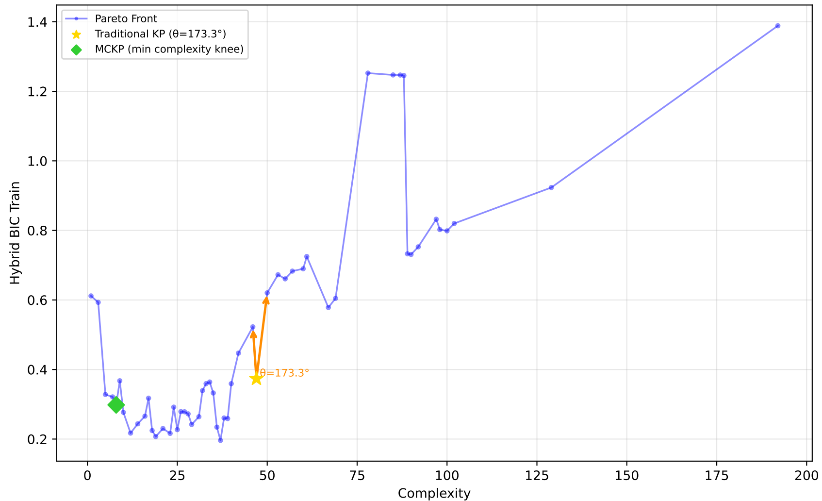
228_elusage - Run 15 - SVP - Hybrid BIC Train \lambda_1=0.00, \lambda_2=1.00, \lambda_3=0.00 | Difficulty: 0.66 | Method: hmr
