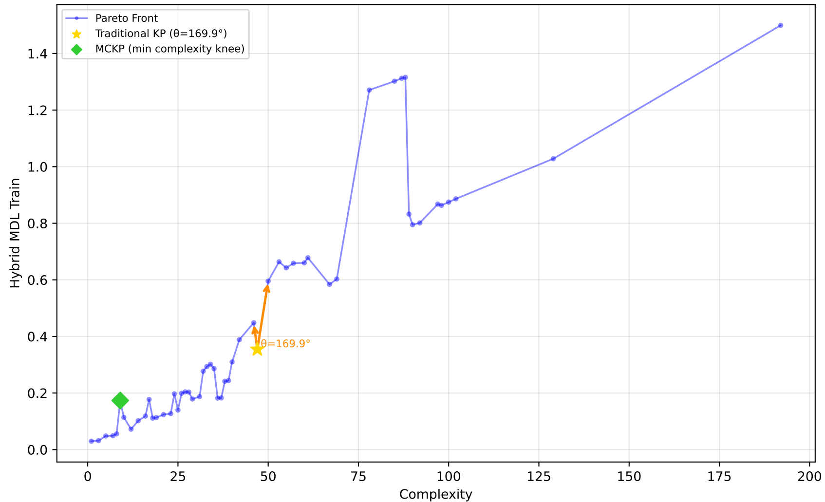
228_elusage - Run 15 - SVP - Hybrid MDL Train \lambda_1=0.00, \bar{\lambda}_2=1.00, \lambda_3=0.00 | Difficulty: 0.66 | Method: hmr
