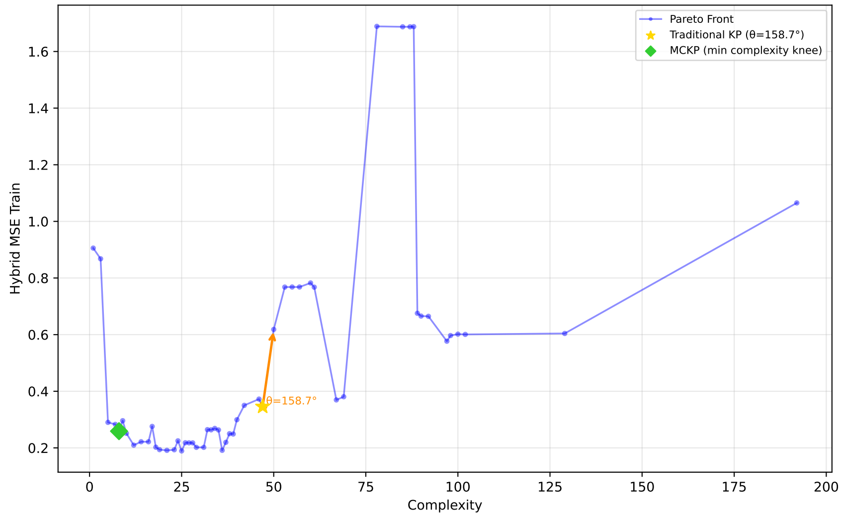
228_elusage - Run 15 - SVP - Hybrid MSE Train \lambda_1=0.60, \bar{\lambda}_2=0.60, \lambda_3=1.00 | Difficulty: 0.66 | Method: hmr
