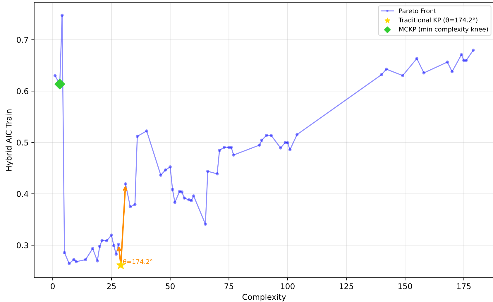
228_elusage - Run 16 - MVP - Hybrid AIC Train \lambda_1=0.00, \lambda_2=0.30, \lambda_3=0.00 | Difficulty: 0.72 | Method: hmr
