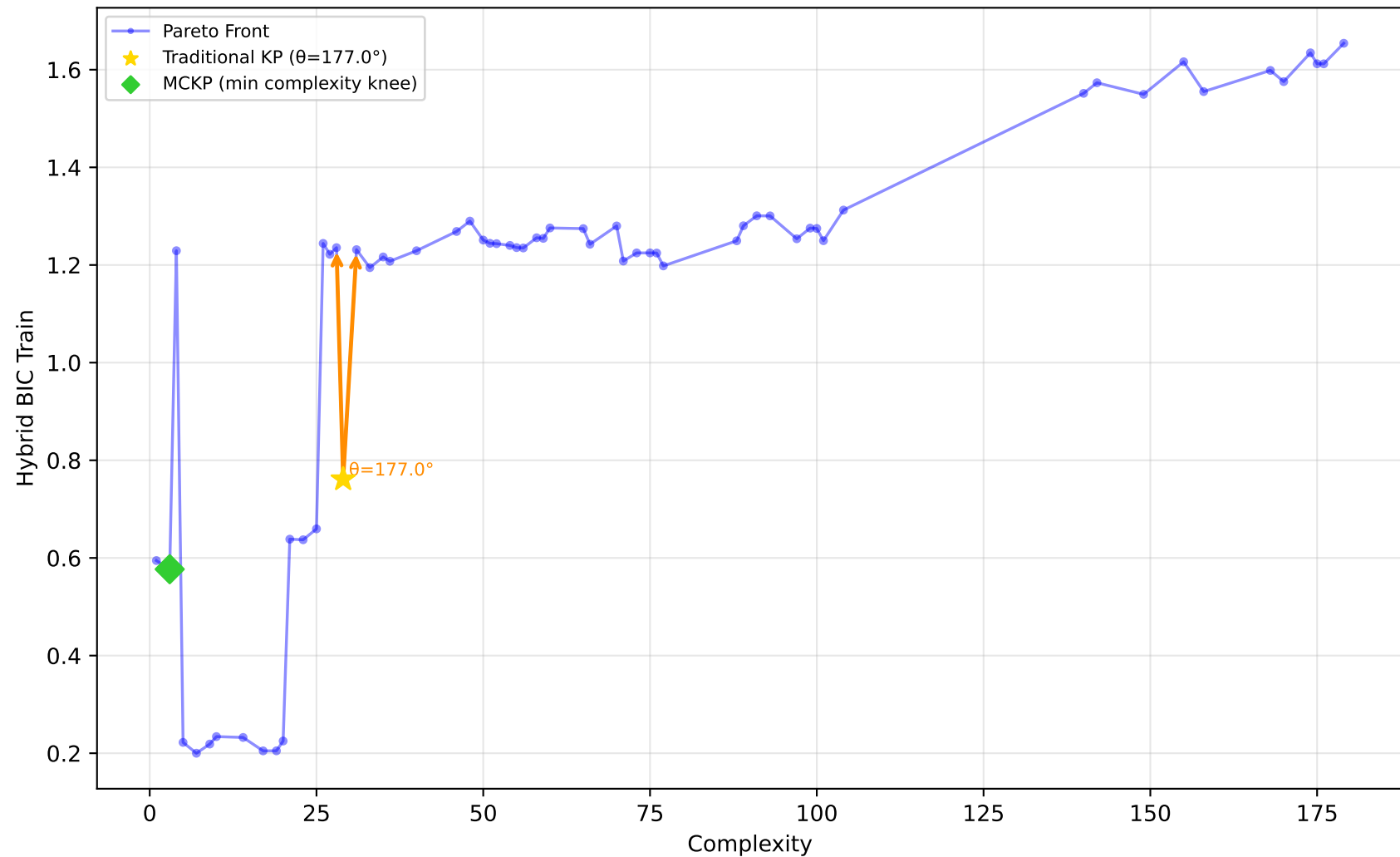
228_elusage - Run 16 - MVP - Hybrid BIC Train \lambda_1=0.00, \bar{\lambda}_2=0.00, \lambda_3=1.00 | Difficulty: 0.72 | Method: hmr
